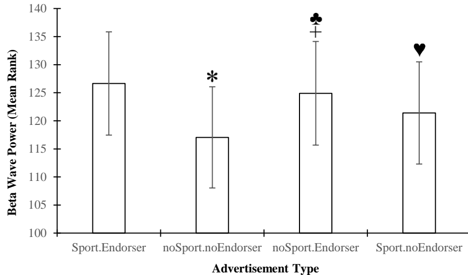
Graph 2. Analysis of Beta Wave Responses of Frontal Cortex to Sports and Non-Sports Product Advertisements with a Sports Endorser. *: Significant difference with Sport.Endorser ( p < 0.001 , 95% CI=[-4.89, -2.23]). +: Significant difference with Sport.Endorser ( p = 0.005 , 95% CI=[-3.22, -0.56]). ♣: Significant difference with noSport.noEndorser ( p = 0.014 , 95% CI=[0.34, 3.00]). ♥: Significant difference with noSport.noEndorser ( p < 0.001 , 95% CI=[1.56, 4.22]).
