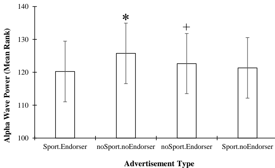
Graph 1. Analysis of Alpha Wave Responses of Frontal Cortex to Sports and Non-Sports Goods Advertisements with a Sports Endorser. *: Significant difference with Sport.Endorser ( p=0.002 , 95% CI=[-3.45, -0.79]). +: Significant difference with Sport.Endorser ( p=0.032 , 95% CI=[-2.56, -0.12]).
